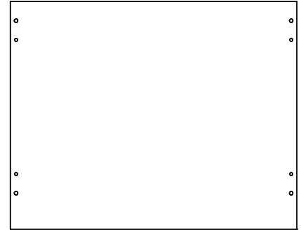
3 (15 x 380 x 478mm) (0,59 x 14,96 x 18,82in)
